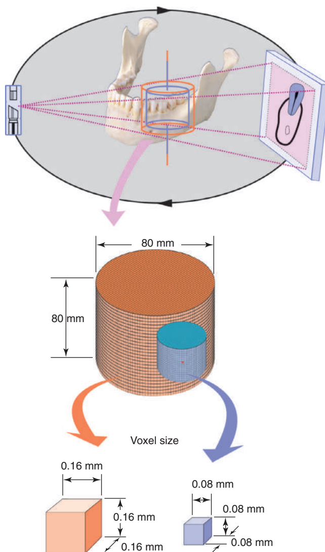
Fig. 1.30 The radiation source in cone-beam volumetric tomography is conical. The receiving sensor captures the image as “voxels,” or three-dimensional pixels of information, allowing digital interpretation.
